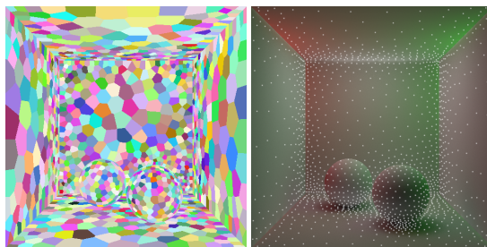
Figure 3: (a) shows our clustering result for the Cornell box scene computed with 1600 clusters; (b) displays the cluster centers on top of a raytraced reference showing the actual irradiance values.
