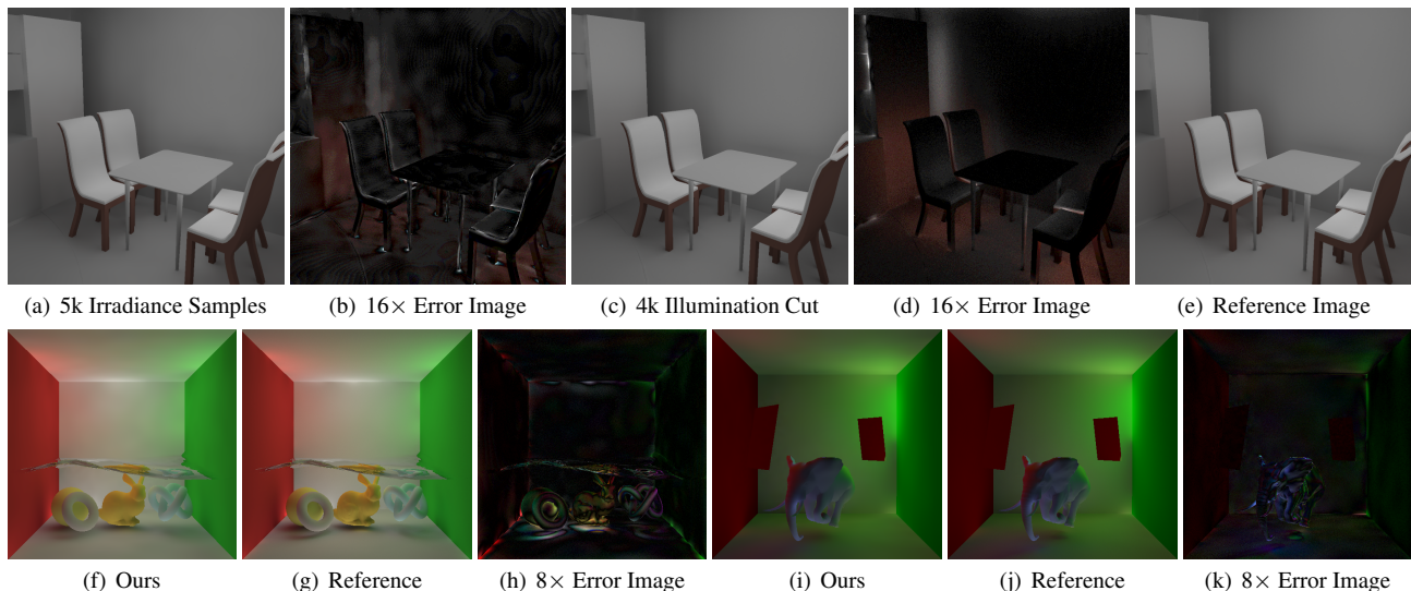
Figure 6: Comparison of indirect illumination results with reference images. The first row shows the kitchen scene: (a) is computed with 5k irradiance samples and the full photon map; (c) is computed at every shading point with an illumination cut size of 4k; (b) and (d) show magnified error images of (a) and (c) against reference (e). The second row shows the same comparison for two additional scenes where the results used for comparison are computed using parameters listed in Table 1.
