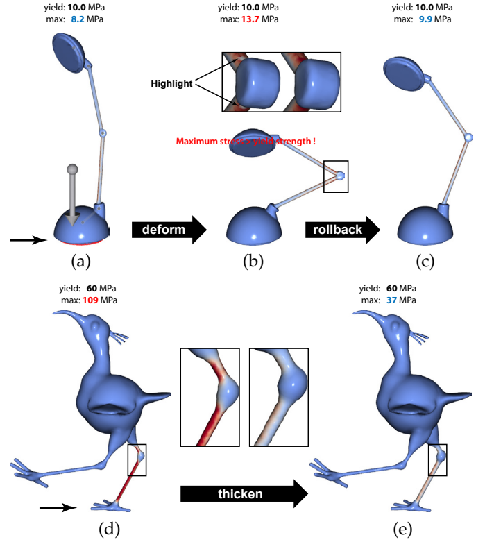
Fig. 14. Stress-aware design. (a) An input shape has a valid stress. (b) The shape is deformed by the user into an invalid pose (i.e., maximum equivalent stress becomes larger than a 10 MPa of yielding strength). (c) Shape rollback operation is triggered to pull the shape back to a valid pose with 9.9 MPa maximum stress. (d) The stress is still too large on the supporting leg. (e) Bone thickening operation is triggered to make the shape valid under a 60 MPa of yielding strength.
